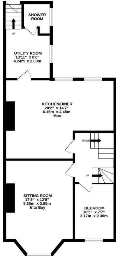
FIRST FLOOR 711 sq.ft. (66.0 sq.m.) approx.
