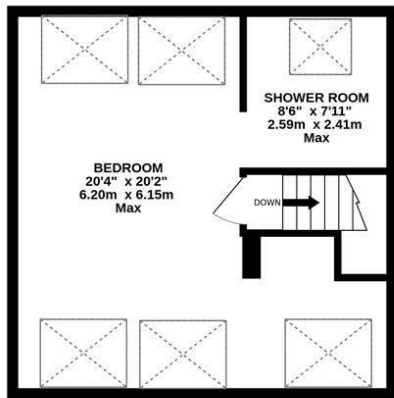
SECOND FLOOR 408 sq.ft. (37.9 sq.m.) approx.
